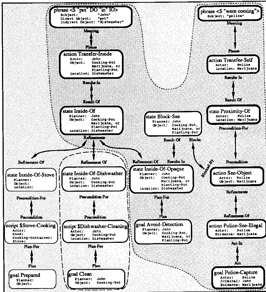
Figure 6. Overview of a small portion of a ROBIN semantic network showing inferences dynamically made after (syntactically pre-processed) input for phrases P1 and P2 of Hiding Pot have been presented. Thickness of frame boundaries shows the amount of evidential activation for the frames. Role fillers have been dynamically instantiated with signature activation. Darkly shaded area indicates the most highly-activated path of nodes representing the most probable plan/goal analysis of the input. Dashed area shows the discarded dishwasher-cleaning interpretation. Nodes outside of both areas show a very small portion of the rest of the network. These nodes received no evidential or signature activation from either phrase.
