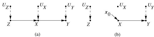
FIG. 2. The diagrams associated with (a) the structural model of equation (2.1) and (b) the modified model of equation (2.2), representing the intervention do(X = x_0) .
