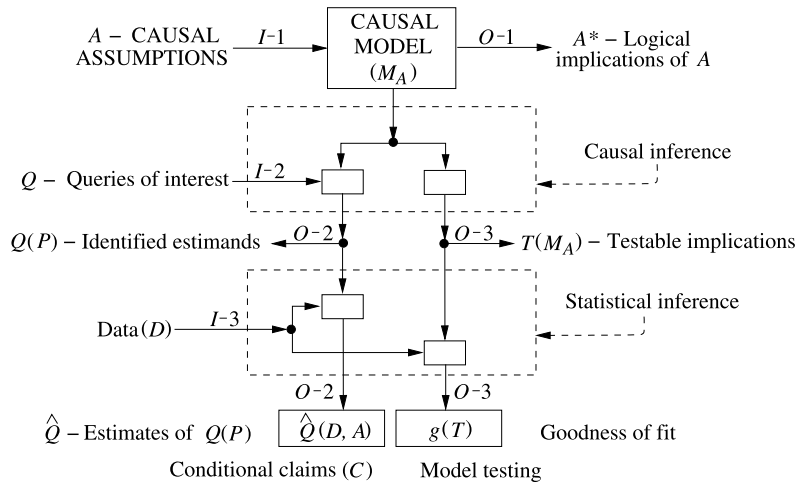
FIG. 1. Causal analysis depicted as an inference engine converting assumptions (A), queries (Q), and data (D) into logical implications (A*), conditional claims (C), and data-fitness indices (g(T)).
