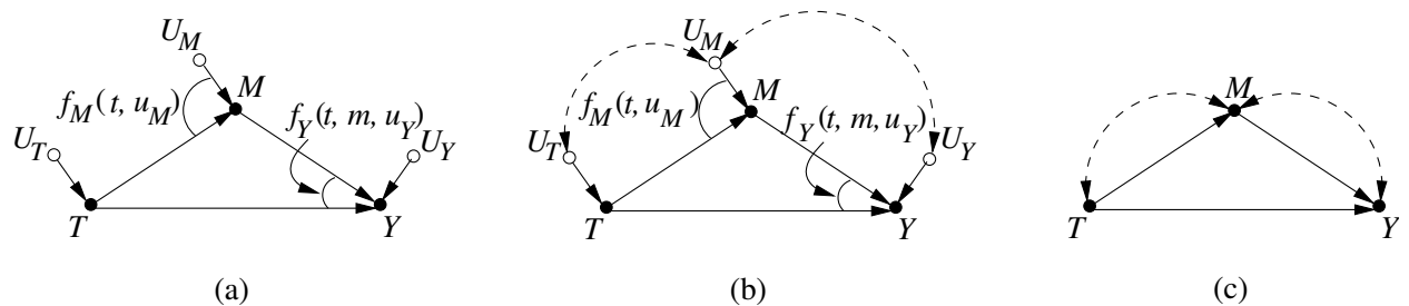
Figure 2: (a) The basic nonparametric mediation model; (b) A confounded mediation model in which dependence exists between U_M and (U_T, U_Y) ; (c) A shorthand notation for (b). M = Mediator; T = Treatment; U = Omitted Factors; Y = Outcome; f = Structural Function; t = Value of T ; u = Value of U ; m = Value of M .
