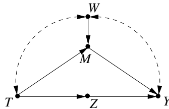
Figure 7: The natural direct effect is identified by adjusting for W and by using Z as auxiliary variable to identify P(y \mid do(t, m), w) as required by A-4 . M = Mediator; T = Treatment; W = Covariate; Y = Outcome; Z = Covariate.
