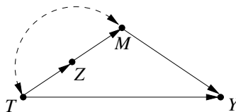
Figure 6: Measuring Z permits the identification of the effect of T on M through the front-door procedure, Eq. (20). Z satisfies the front-door condition since it intercepts all paths from T to M , and receives no other arrow except for T \rightarrow Z . M = Mediator; T = Treatment; Y = Outcome; Z = Covariate.
