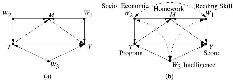
Figure 3: (a) A mediation model with three independent confounders, permitting the decomposition of Eq. (18). (b) A model with dependent deconfounders, satisfying conditions A and B . M = Mediator; T = Treatment; W = Covariates; Y = Outcome.
