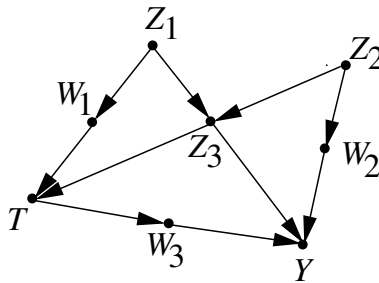
Figure 12: Graphical model illustrating the backdoor criterion. Error terms are not shown explicitly. T = Treatment; W = Covariates; Y = Outcome; Z = Covariates.
