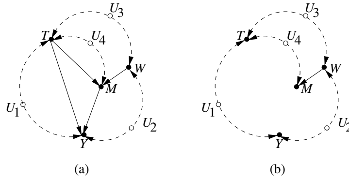
Figure 13: (a) A causal model with latent variables ( U_s ) where the natural direct effect can be identified in experimental studies. (b) The subgraph G_{T,M} illustrating the criterion of experimental identifiability (Eq. 40): W d -separates Y from \overline{M} . M = Mediator; T = Treatment; W = Covariate; Y = Outcome; U = Omitted Factors.
