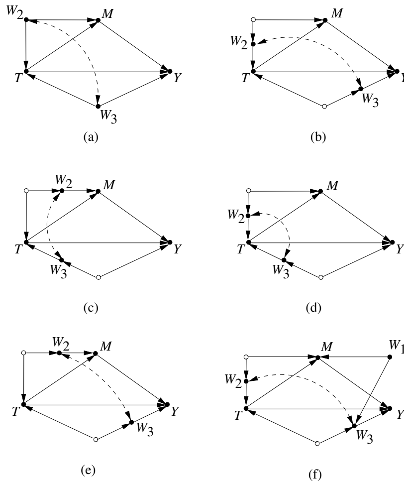
Figure 5: Showing six confounded models for comparing assumption sets A and B . The former is satisfied in all cases except (d); the latter is satisfied in (a) and (e) only. Explanations are given in Table 2. M = Mediator; T = Treatment; W = Covariates; Y = Outcome.
