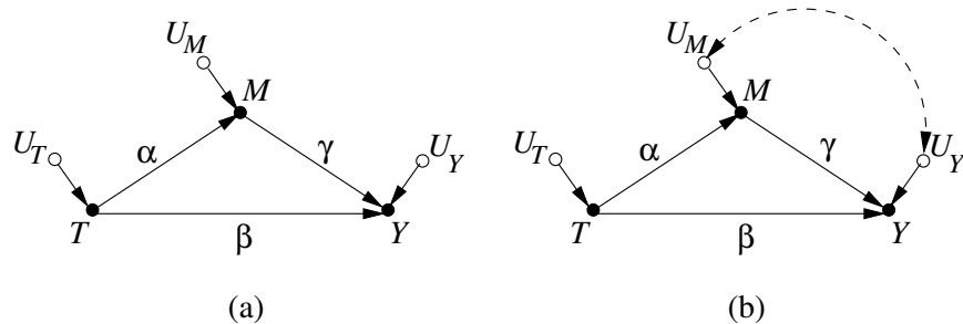
Figure 1: (a) The basic (unconfounded) mediation model. (b) A confounded version of (a), showing correlation between U_M and U_Y . Solid bullets represent observed variables, hollow circles represent unobserved (or latent) variables. M = Mediator; T = Treatment; Y = Outcome; U = Omitted Factors; \alpha = T - M Effect Coefficient; \beta = Direct T - Y Effect Coefficient; \gamma = M - Y Effect Coefficient; f = Structural Function; t = Value of T ; m = value of M .
