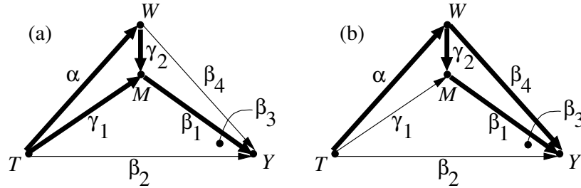
Figure 11: A parameterized version of Fig. 10, in which the heavy arrows represent (a) Paths carrying the natural indirect effect ( NIE ) when M is considered as the mediator. (b) Same with W considered as the mediator. M = Mediator; T = Treatment; W = Covariate; Y = Outcome; \alpha, \beta, \gamma = Structural Coefficients.
