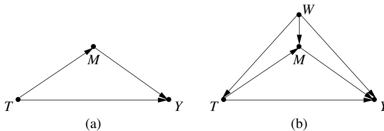
Figure 4: (a) The basic unconfounded mediation model, (same as Fig. 1(b), with omitted factors not shown). (b) A confounded mediation model with covariate set W that deconfounds both the T \rightarrow M, T \rightarrow Y and the M \rightarrow Y relationships. M = Mediator; T = Treatment; W = Covariate; Y = Outcome.
